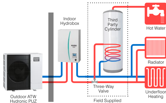
ATW Hydronic Hydrobox System
